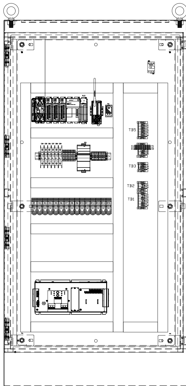
BACK PANEL VIEW
